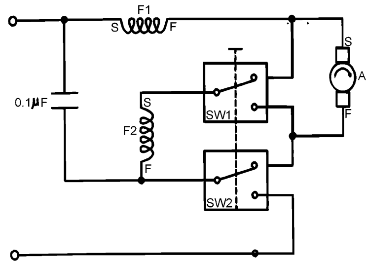
CIRCUIT DIAGRAM FOR BRAKED UNITS
