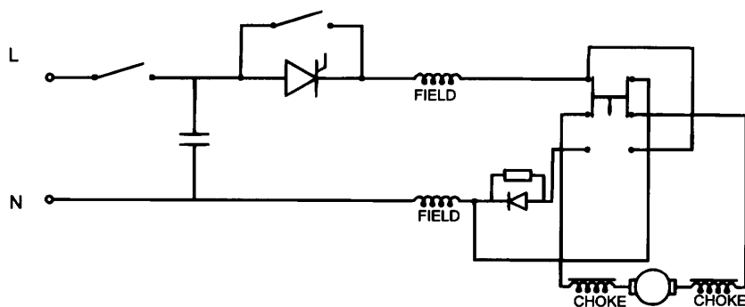
CIRCUIT DIAGRAM
