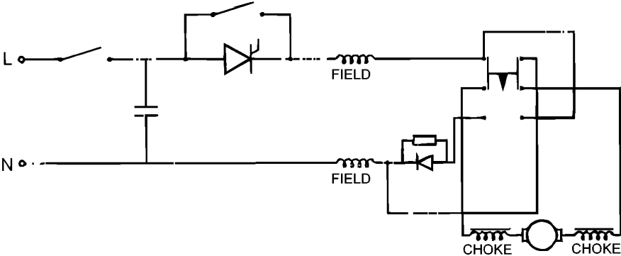
VARIABLE SPEED REVERSING UNITS
