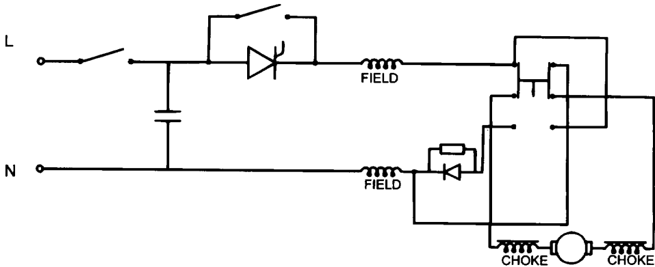
CIRCUIT DIAGRAM
