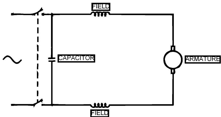
CIRCUIT DIAGRAM
