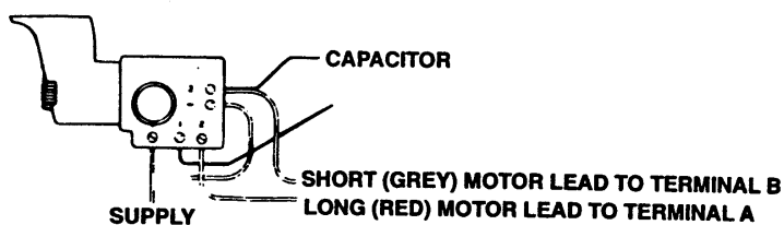
SWITCH WIRING DIAGRAM
